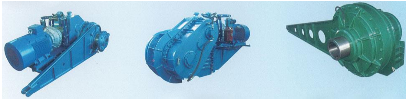
Gearbox for bucket wheel stacker reclaimer
